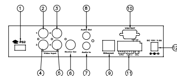
Back Panel Layout
